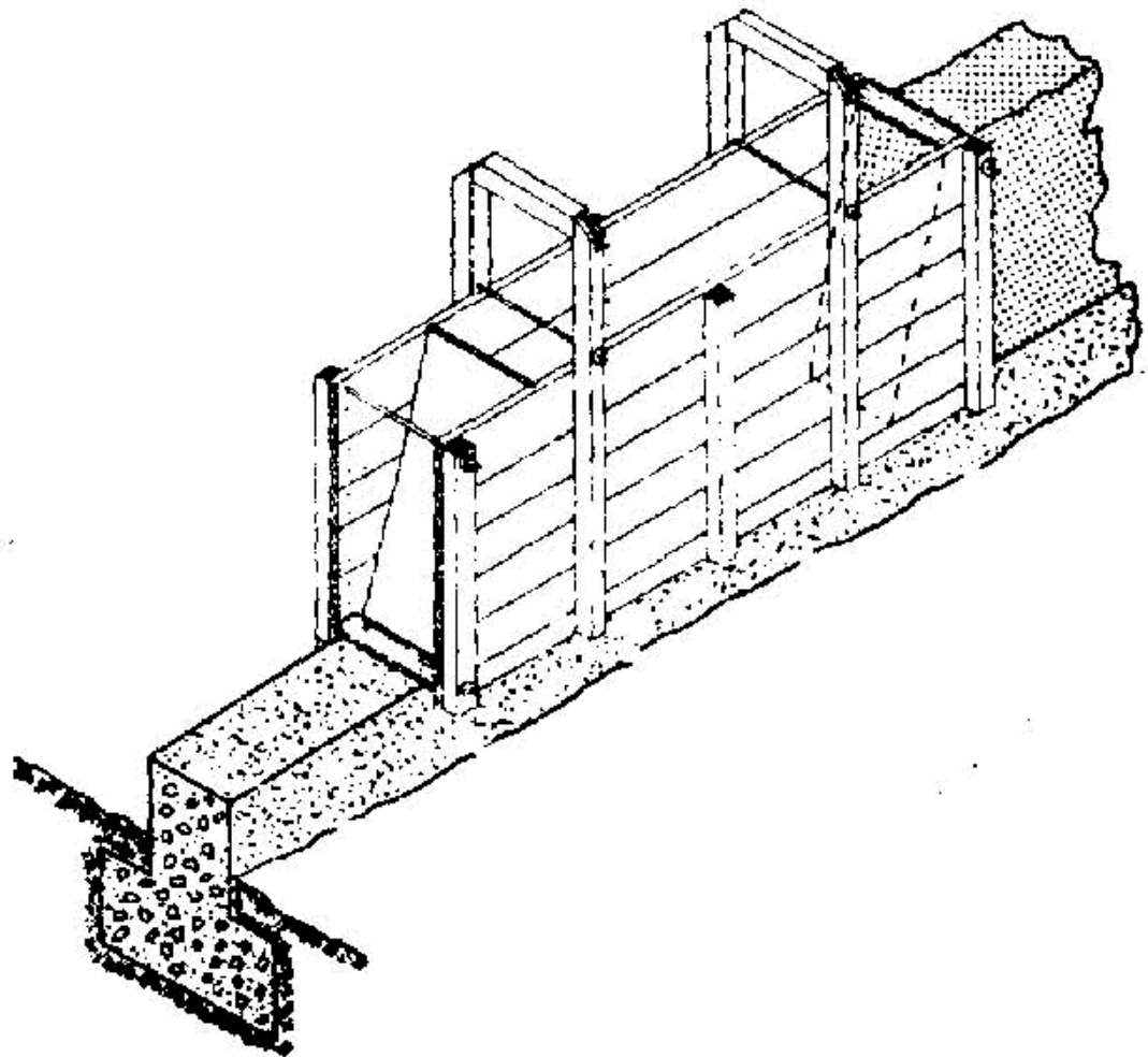
Figure 77. Form for ramming.
