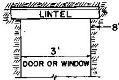
Figure 95. Wood lintel.
